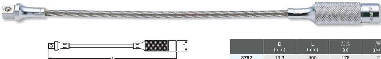
3762 Flexible Extension Bar Alargadera Flexible
