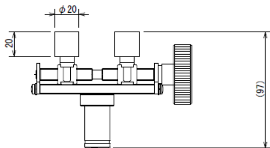
The dimension at mounting the pins
